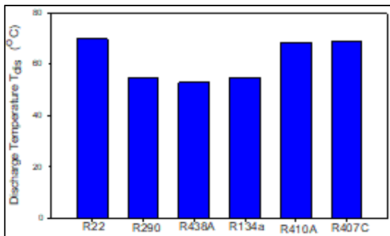
Fig 6: Comparison of Discharge Temperature Stability.
